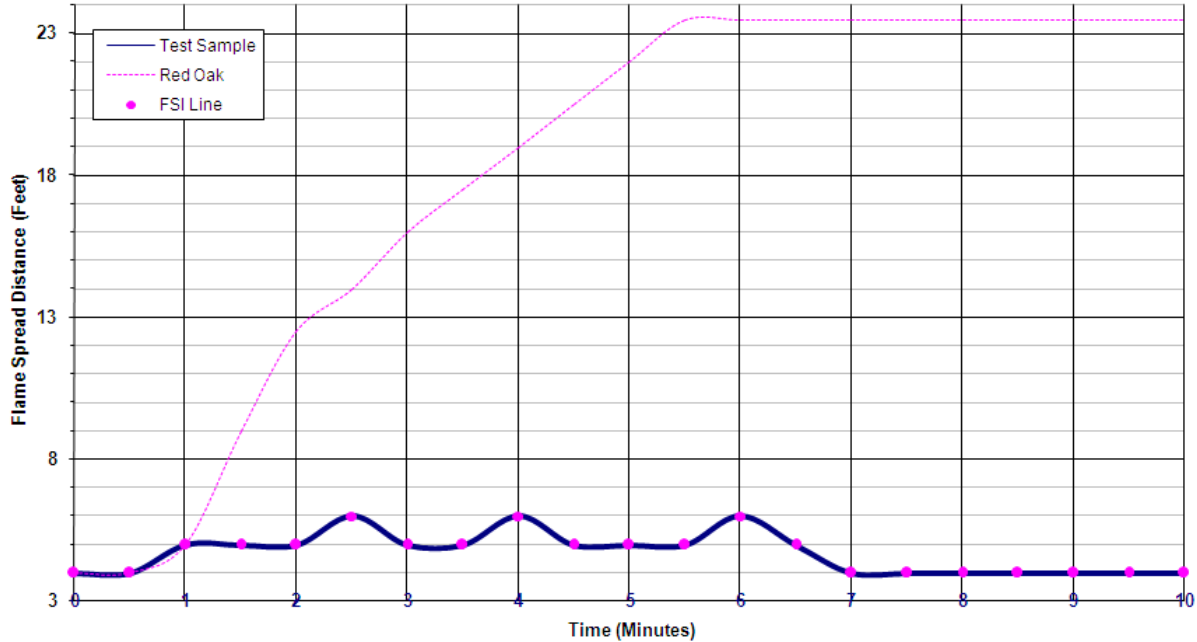
Figure 1. Flame Spread Chart
