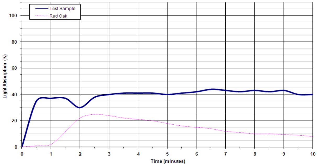
Figure 2. Smoke Developed Chart
